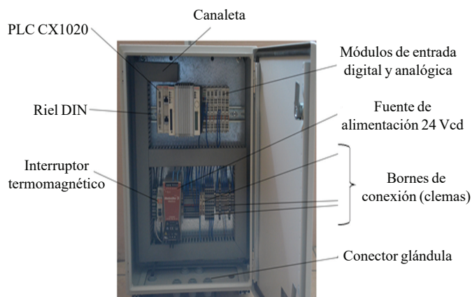
Figura 2. Componentes en gabinete de control (vista interna). Figure 2. Components in the control cabinet (internal view).
